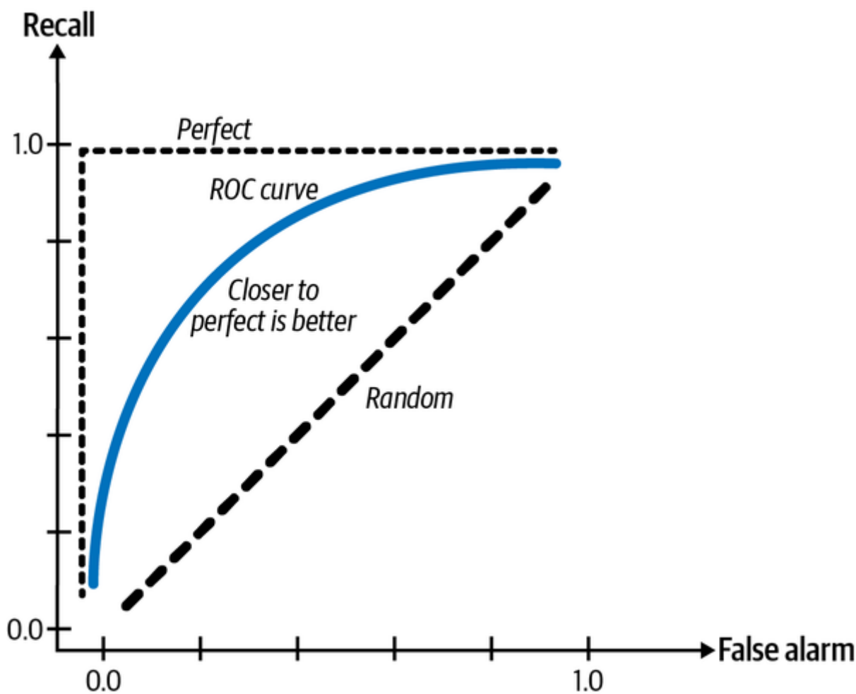
Figure 4-9. ROC curve
