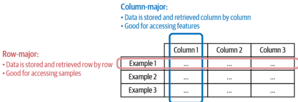
Figure 3-1. Row-major versus column-major formats
