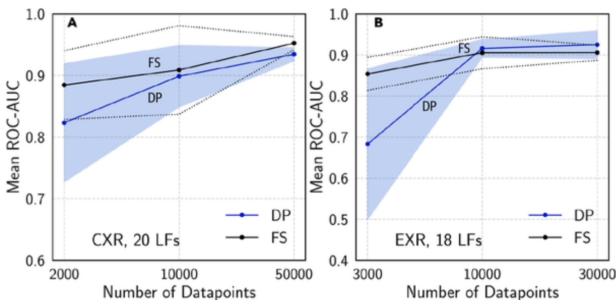
Figure 4-5. Comparison of the performance of a model trained on fully supervised labels (FS) and a model trained with programmatic labels (DP) on CXR and EXR tasks. Source: Dunnmon et al. 15
