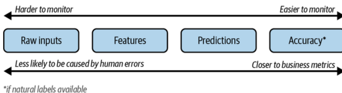
*if natural labels available Figure 8-5. The more transformations an artifact has gone through, the more likely its changes are to be caused by errors in one of those transformations
