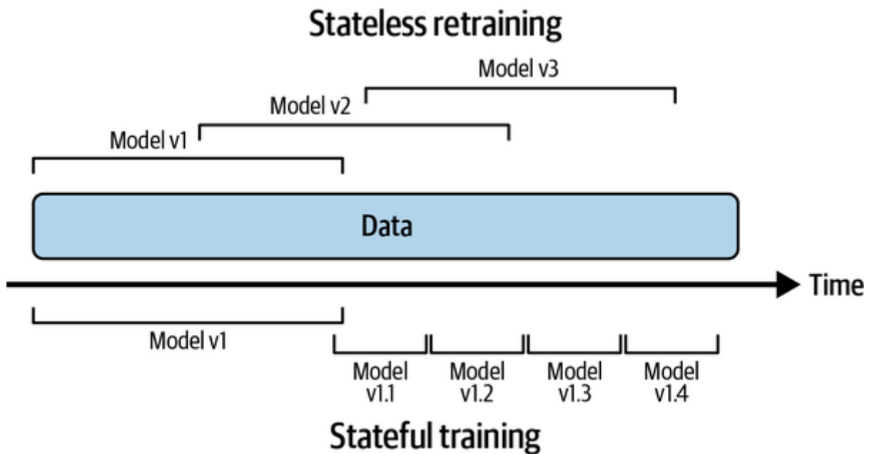
Figure 9-2. Stateless retraining versus stateful training
