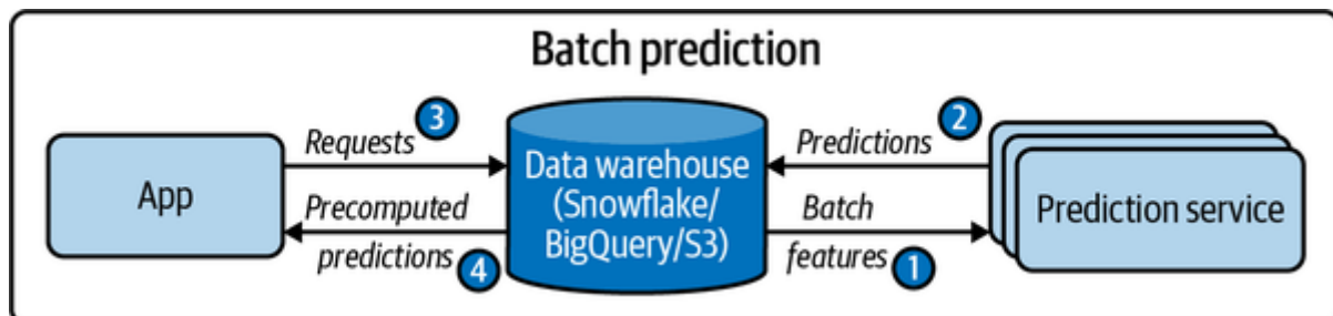
Figure 7-4. A simplified architecture for batch prediction
