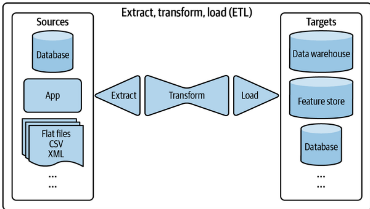
Figure 3-7. An overview of the ETL process
