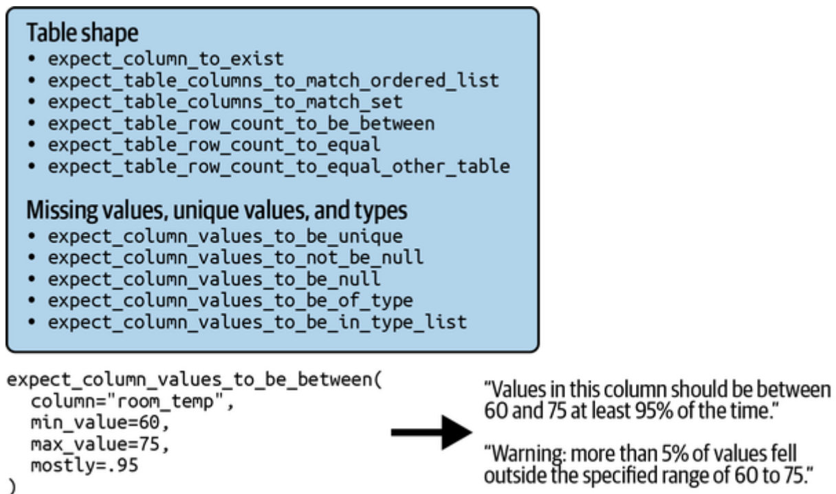
Figure 8-7. Some of the built-in feature validation functions by Great Expectations and an example of how to use them. Source: Adapted from content in the Great Expectations GitHub repository
