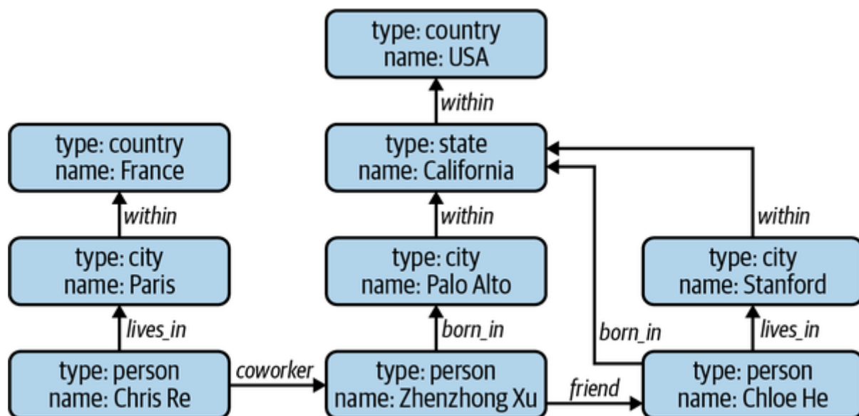
Figure 3-5. An example of a simple graph database
